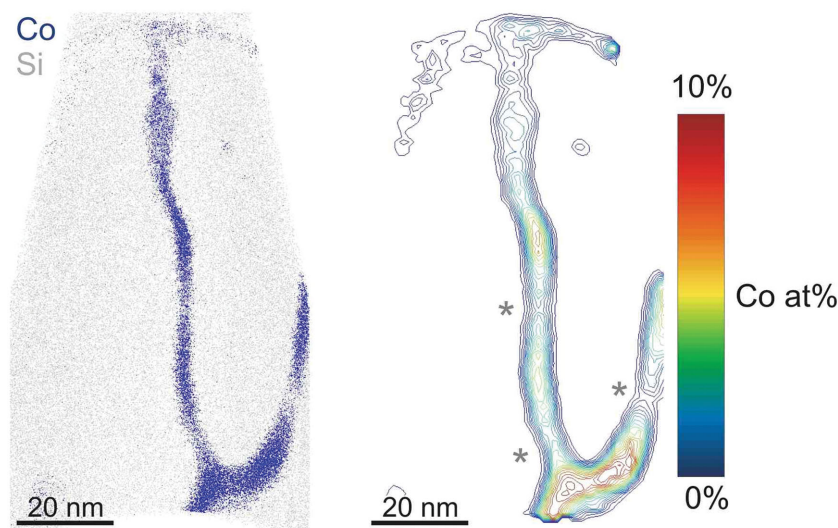
Figure 4. Left, a cross-sectional 15 nm thick slice from an APT dataset, fully enclosing one filamentary breakdown region. Gray atoms denote Si (1% shown for clarity) while blue atoms denote Co (100% shown). A small ( \approx 2 nm) layer of amorphous Si capping material is shown at the top of the image, above the original wafer surface. Right, a 2D Co atomic concentration isocontour plot, with contours in 1 atomic % increments. Asterisks indicate regions of filament where the composition gradient qualitatively resembles “pinch-off” morphology.
