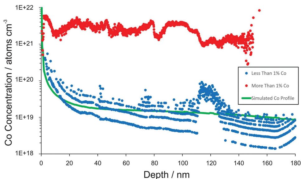
Figure 5. 1D composition versus depth profiles of the decomposed APT dataset. In red, the portion of the data enclosed by a 1% atomic Co concentration isosurface. In blue, the remaining dataset outside of that surface (not including the capping material). In green, a simulation as described by Bom et al. [24] in the main text, with a one-parameter fit to the blue curve. Note that the \gamma -axis striation of the blue curve is the result of single-Co-atom differences within the thin z-sections used to calculate this profile.
